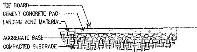
SHOT PUT PAD SECTION A-A
